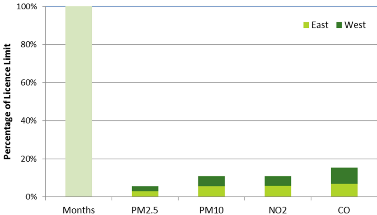
Figure 20: Ventilation Stack Emissions as Percentage of Licence Limit (1/07/2013 - 30/06/2014)
