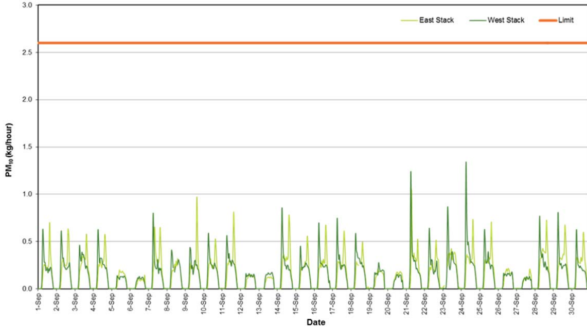
Figure 15: PM 10 Mass Rate (1 Hour Average)
