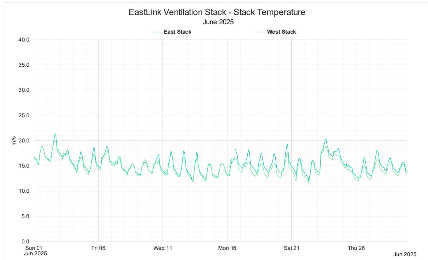
Figure 22: June 2025 Monthly 1-hour average stack temperature
