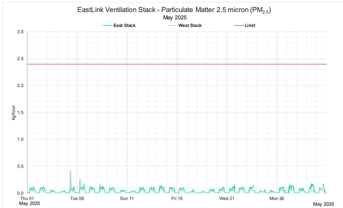
Figure 12: May 2025 Monthly 1-hour mass rate PM_{2.5}
