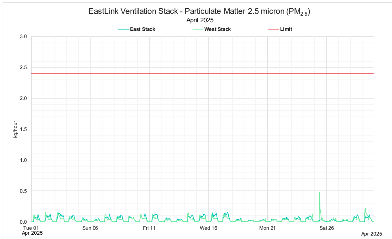
Figure 5: April 2025 Monthly 1-hour mass rate PM 2.5
