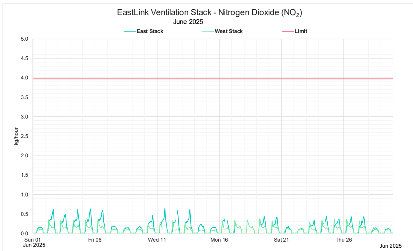
Figure 16: June 2025 Monthly 1-hour mass rate NO 2
