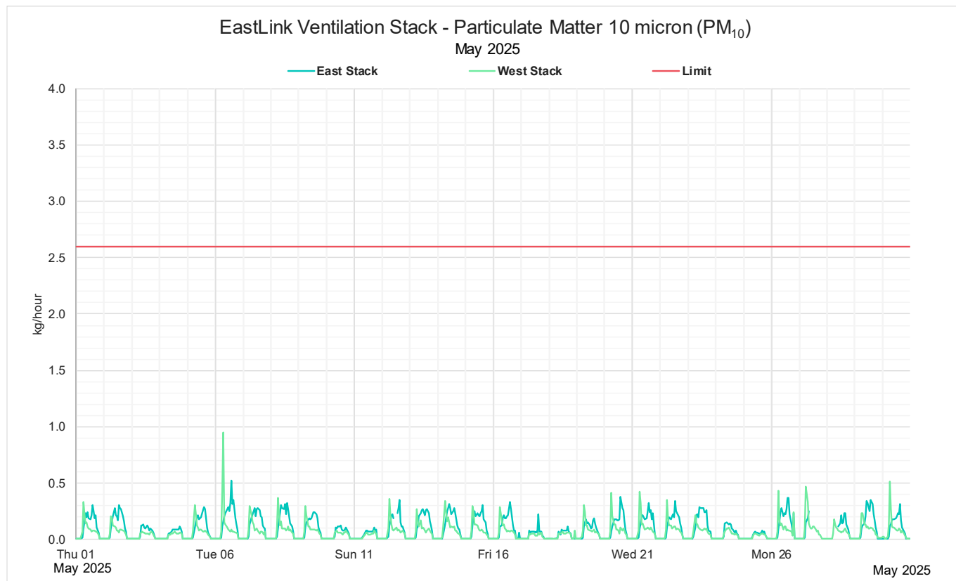
Figure 13: May 2025 Monthly 1-hour mass rate PM_{10}
