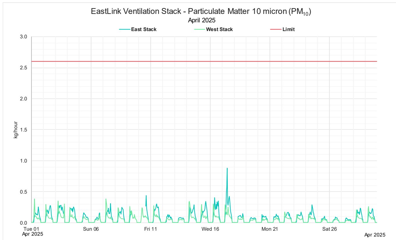
Figure 6: April 2025 Monthly 1-hour mass rate PM 10
