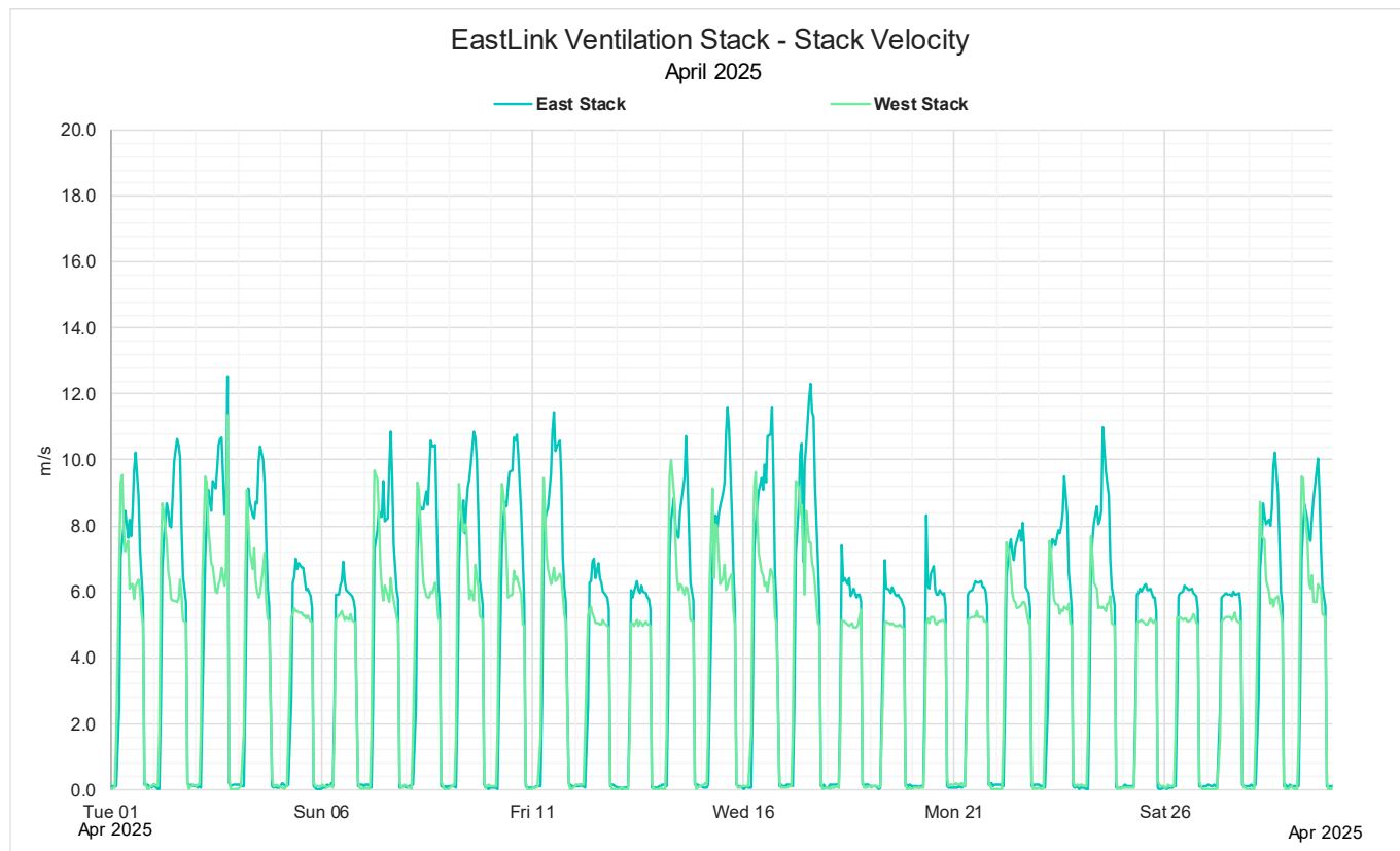
Figure 7: April 2025 Monthly 1-hour average stack velocity
