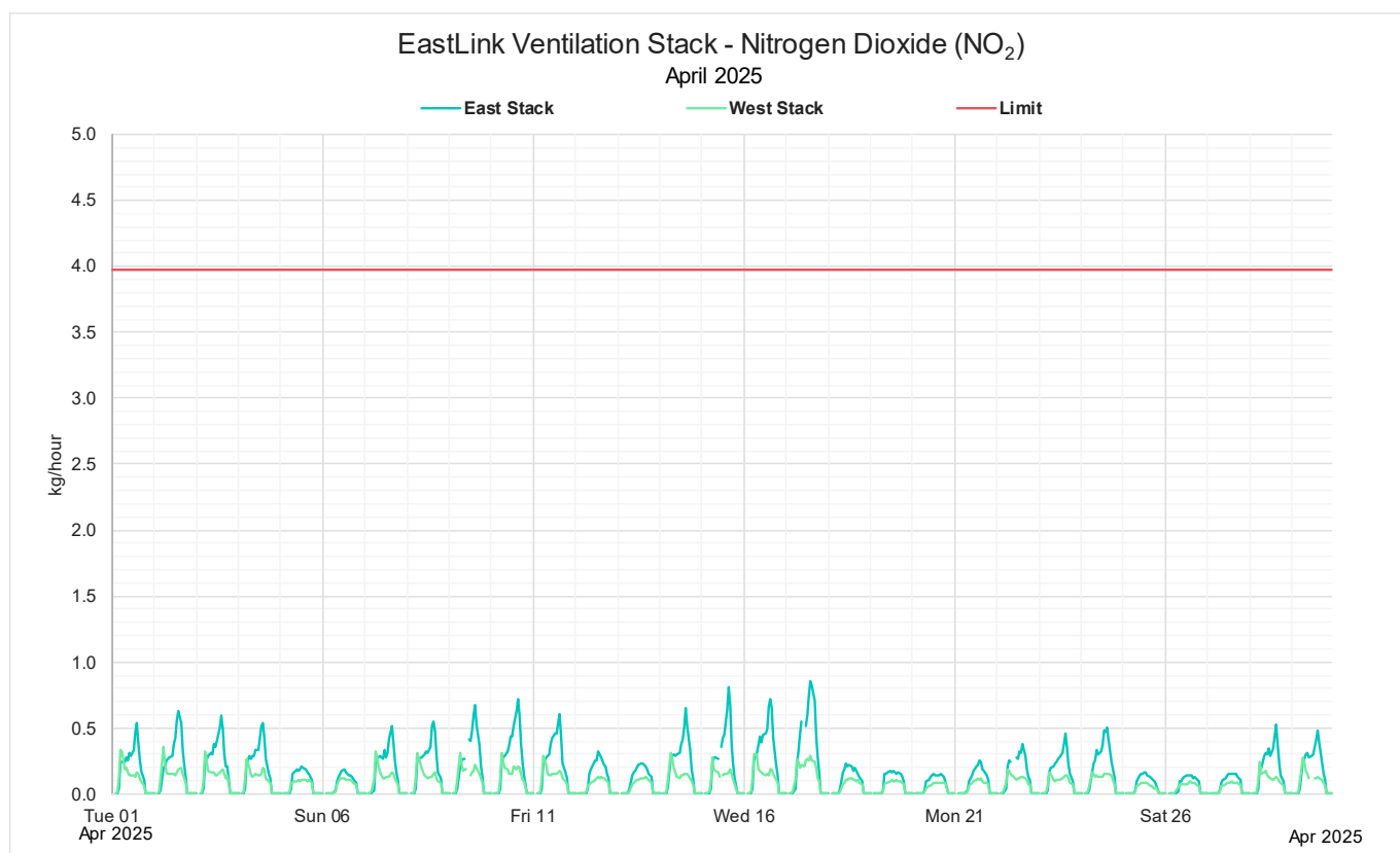
Figure 2: April 2025 Monthly 1-hour mass rate NO 2
