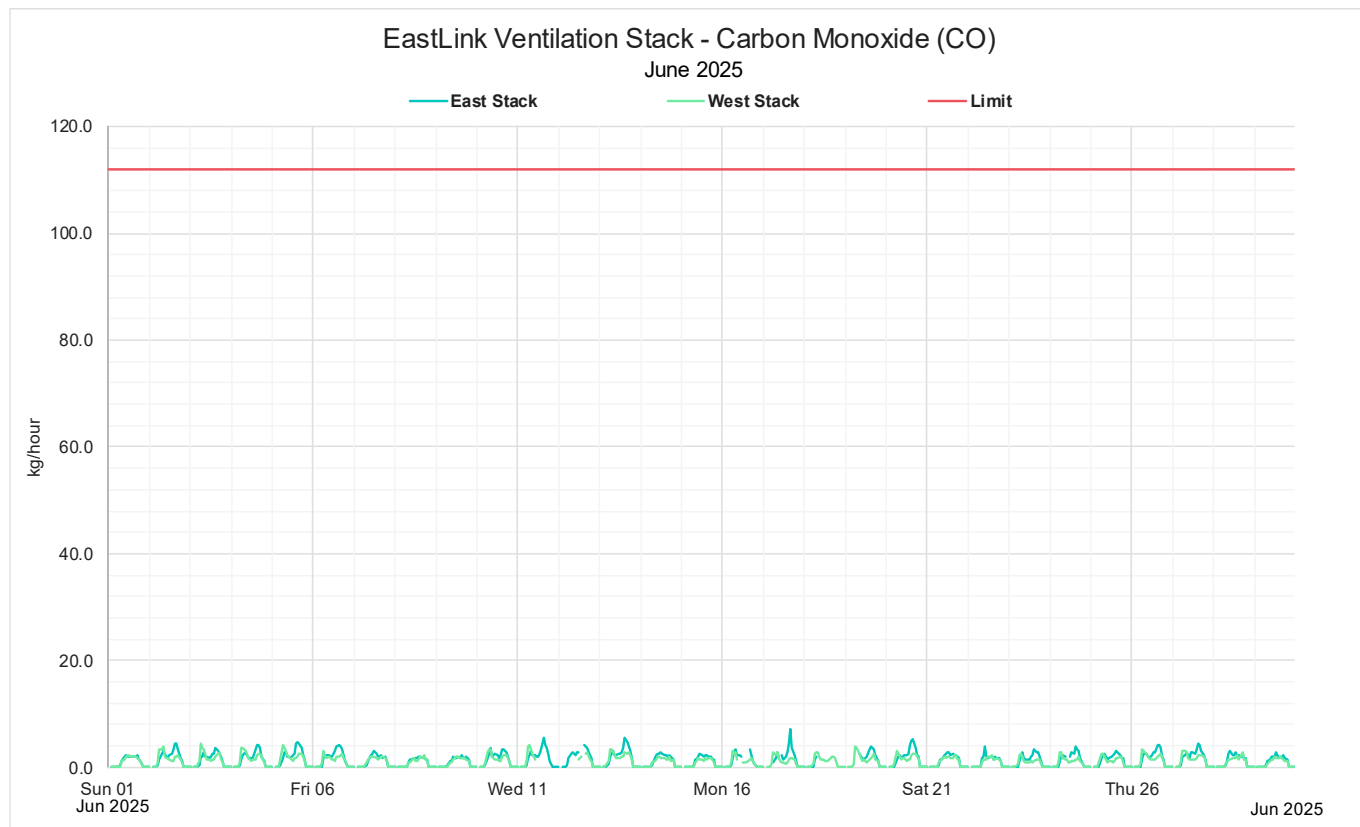
Figure 18: June 2025 Monthly 1-hour mass rate CO
