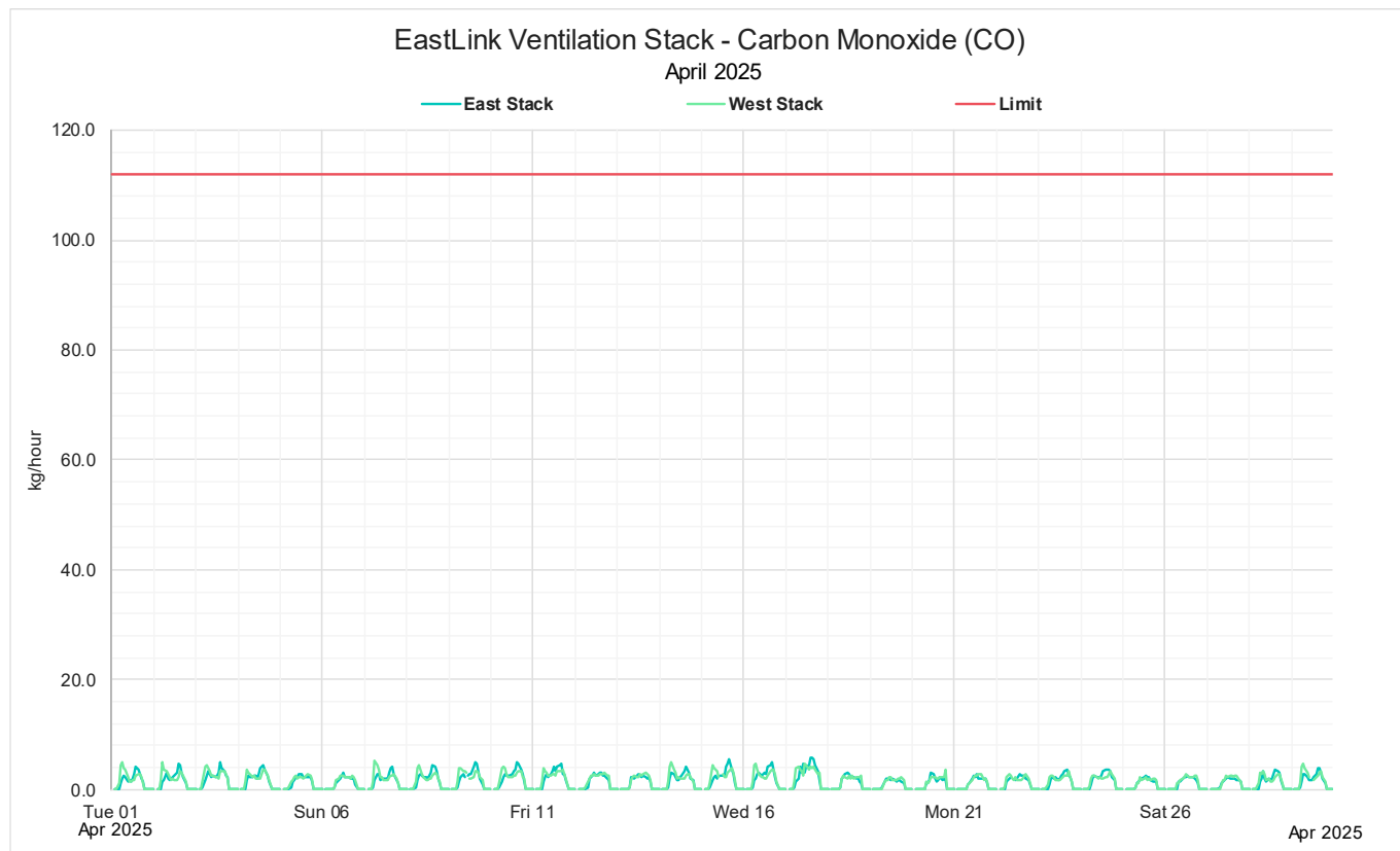
Figure 4: April 2025 Monthly 1-hour mass rate CO
