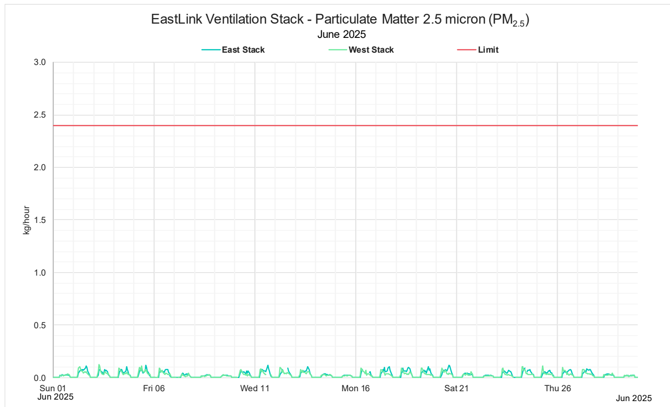
Figure 19: June 2025 Monthly 1-hour mass rate PM_{2.5}
