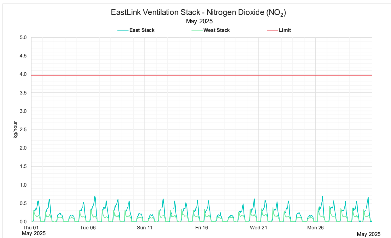
Figure 9: May 2025 Monthly 1-hour mass rate NO 2
