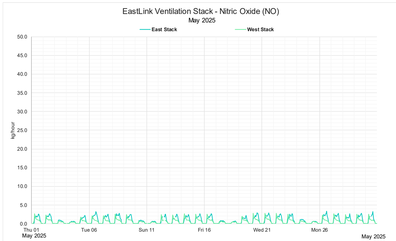
Figure 10: May 2025 Monthly 1-hour mass rate NO
