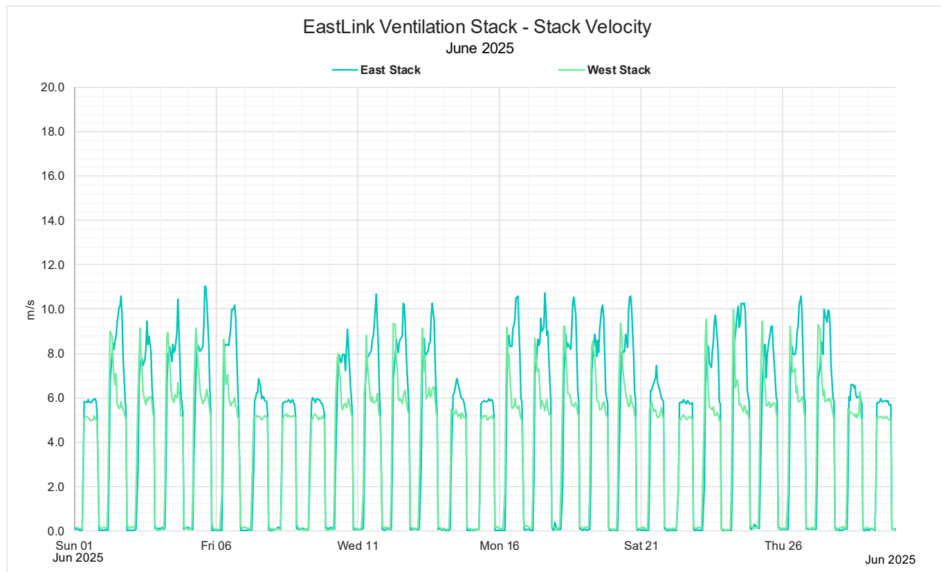
Figure 21: June 2025 Monthly 1-hour average stack velocity
