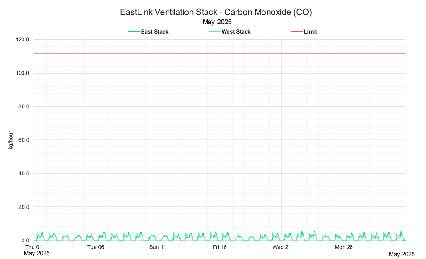
Figure 11: May 2025 Monthly 1-hour mass rate CO
