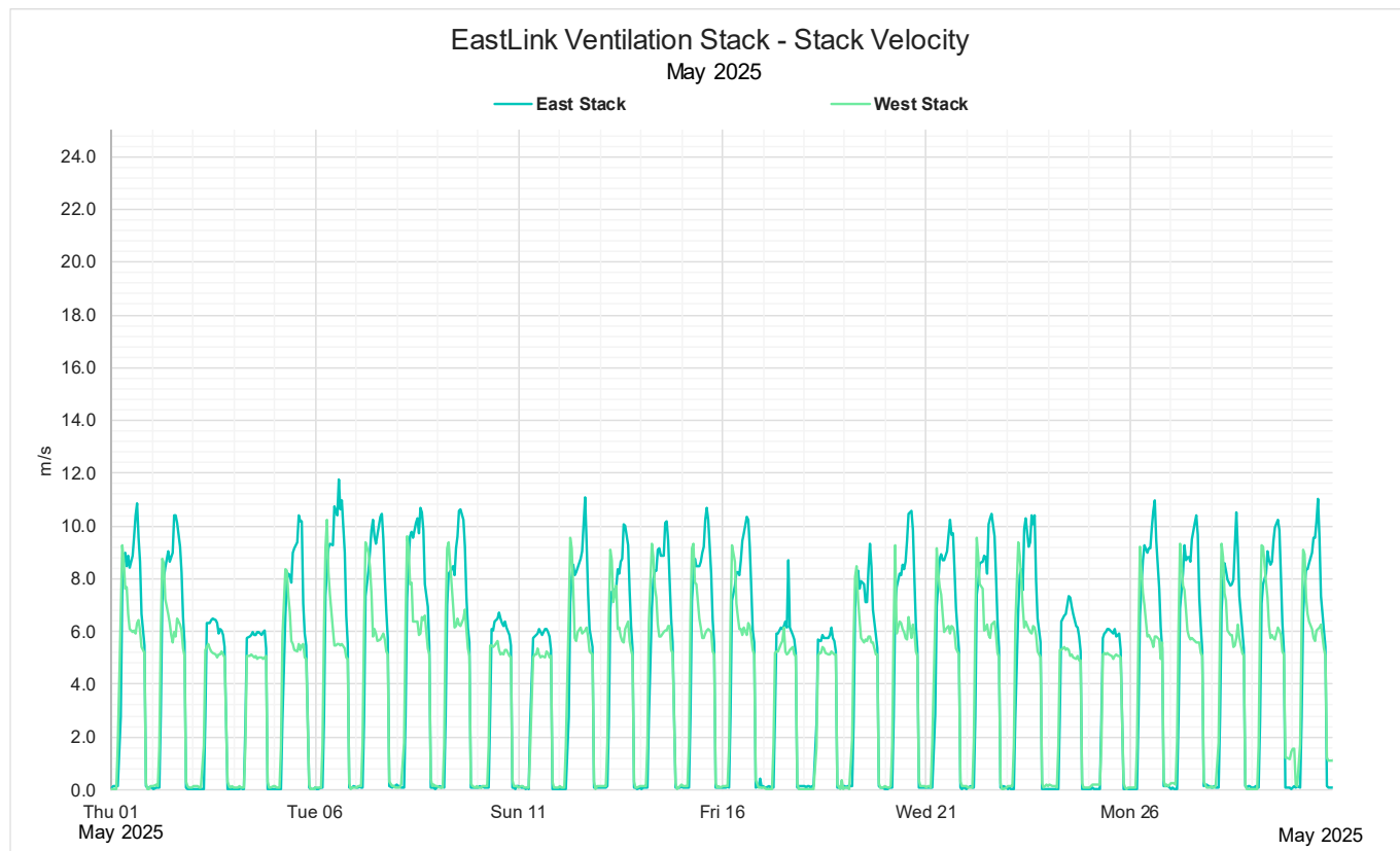
Figure 14: May 2025 Monthly 1-hour average stack velocity
