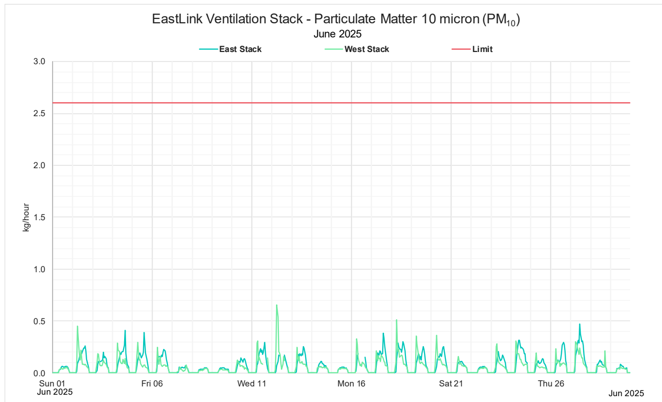
Figure 20: June 2025 Monthly 1-hour mass rate PM_{10}
