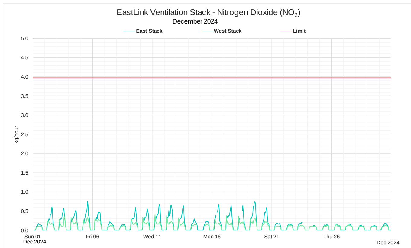
Figure 16: December 2024 Monthly 1-hour mass rate NO 2
