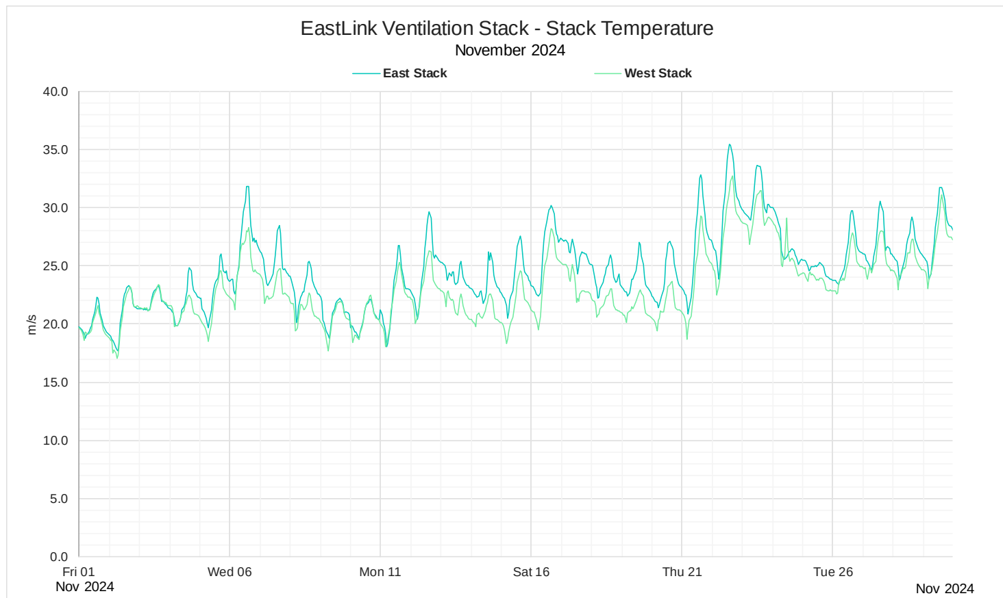
Figure 15: November 2024 Monthly 1-hour average stack temperature
