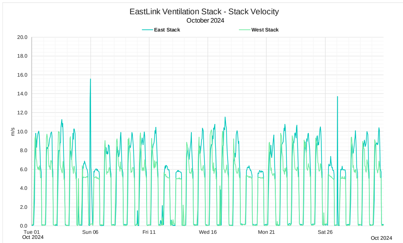
Figure 7: October 2024 Monthly 1-hour average stack velocity
