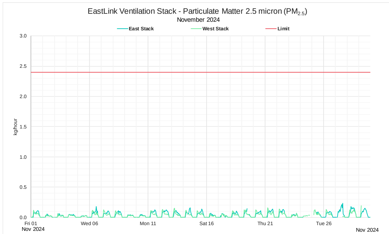
Figure 12: November 2024 Monthly 1-hour mass rate PM 2.5
