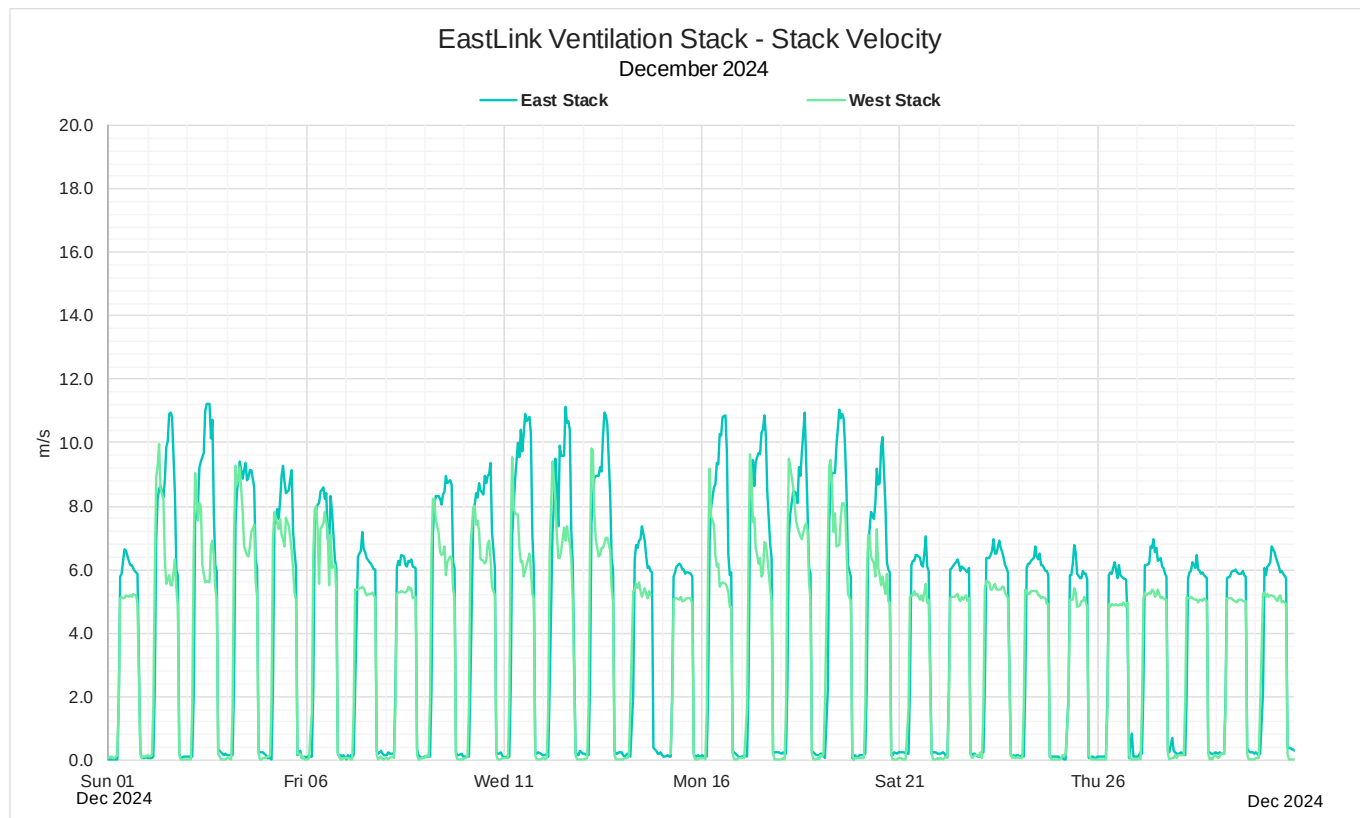
Figure 21: December 2024 Monthly 1-hour average stack velocity
