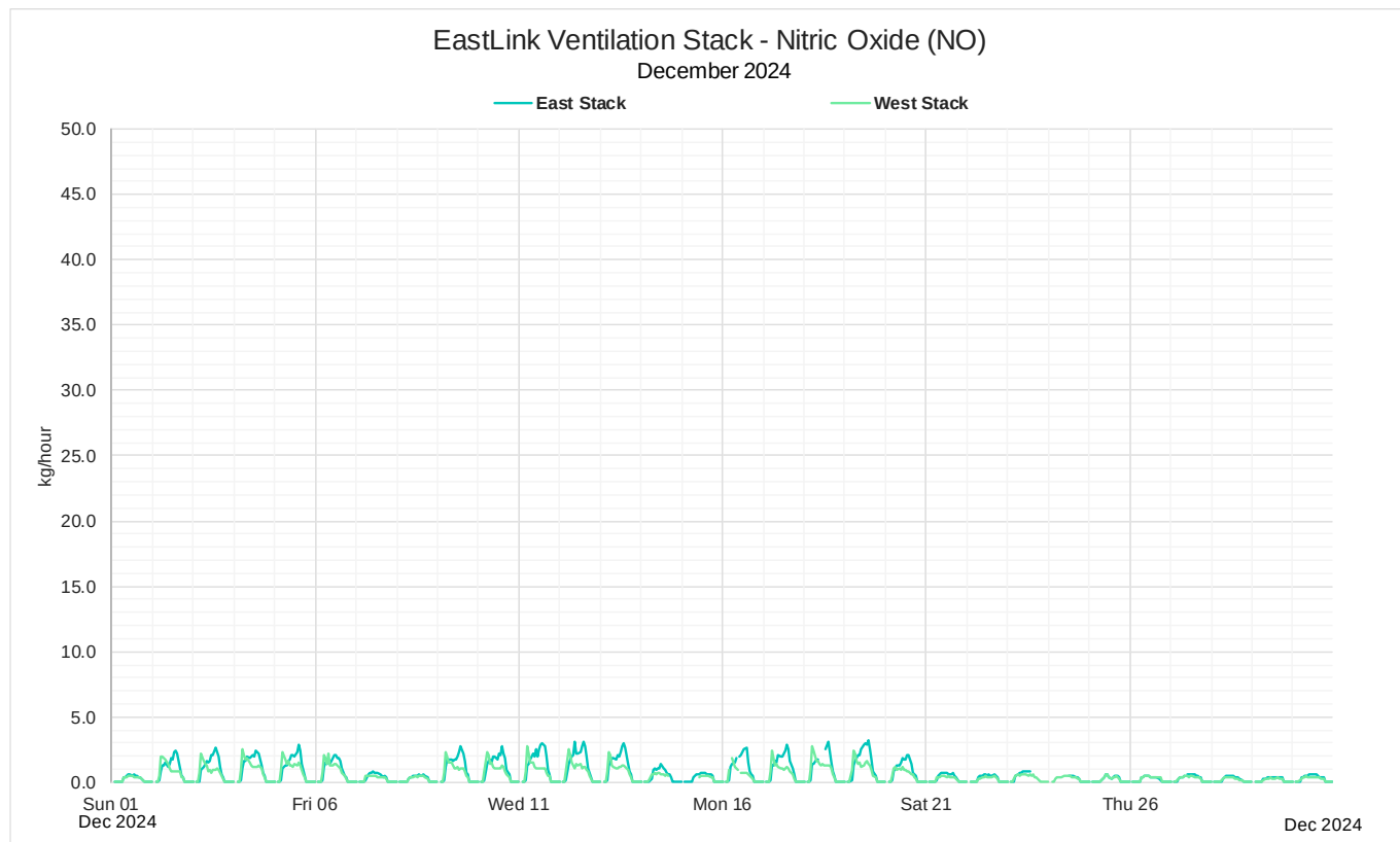
Figure 17: December 2024 Monthly 1-hour mass rate NO
