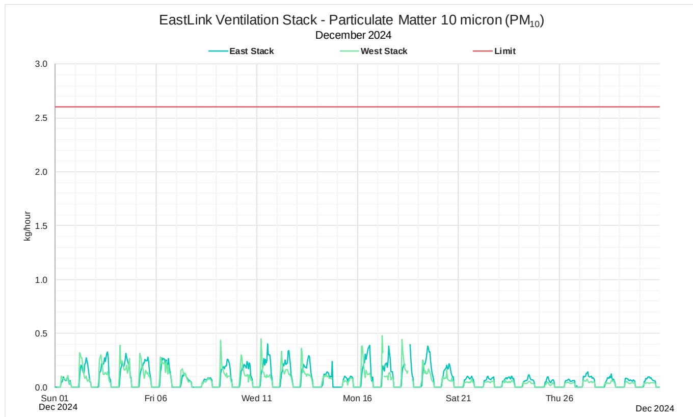
Figure 20: December 2024 Monthly 1-hour mass rate PM_{10}
