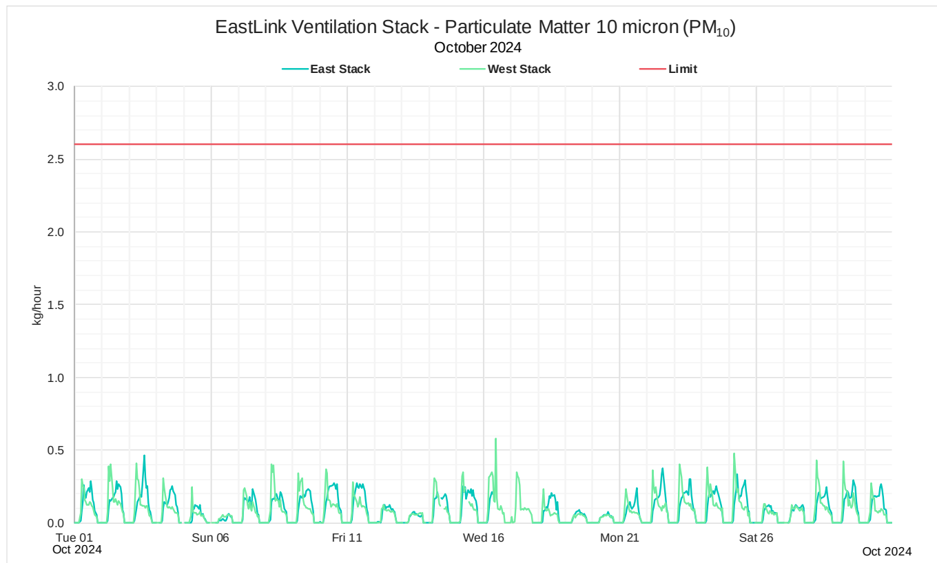
Figure 6: October 2024 Monthly 1-hour mass rate PM 10
