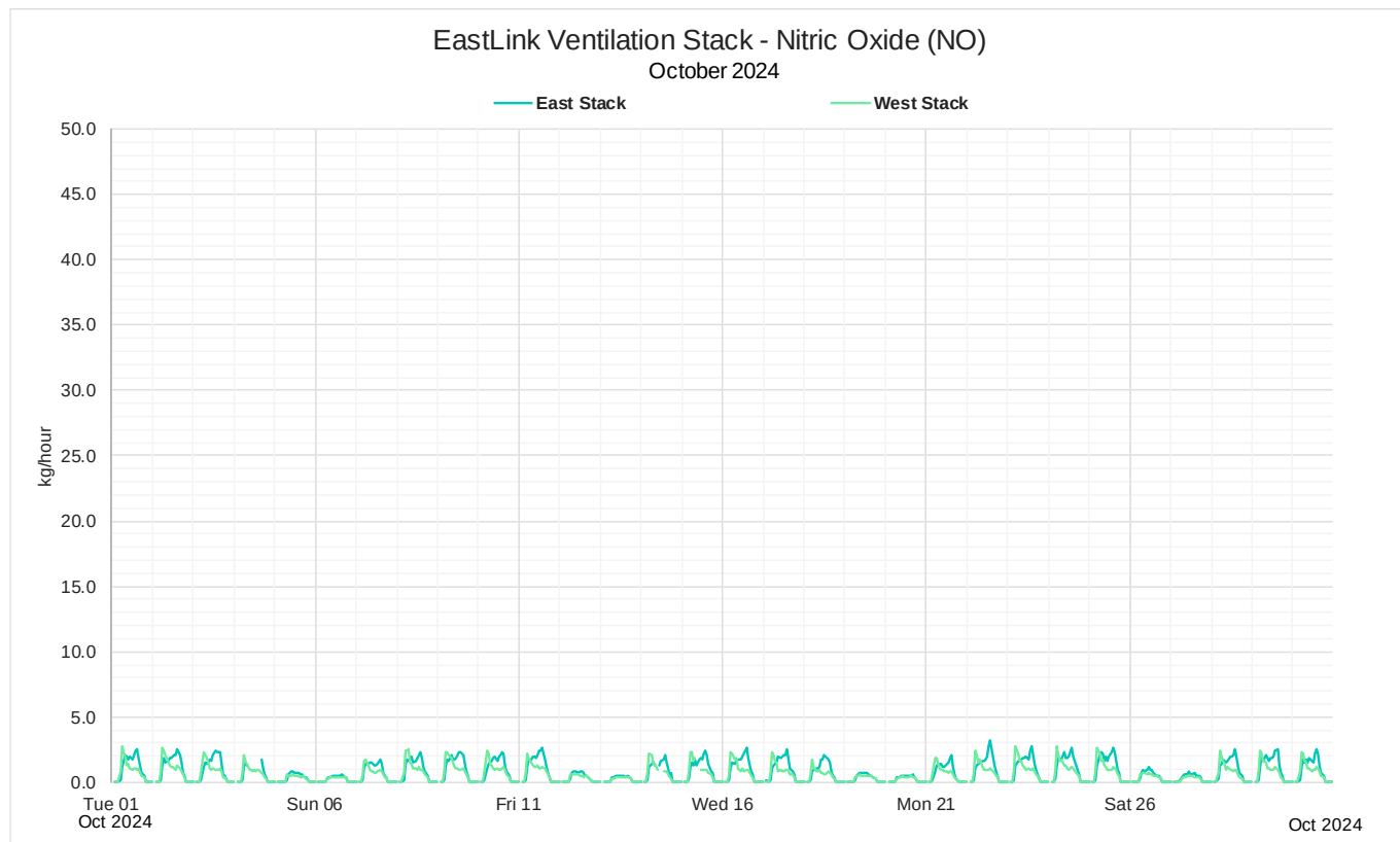
Figure 3: October 2024 Monthly 1-hour mass rate NO
