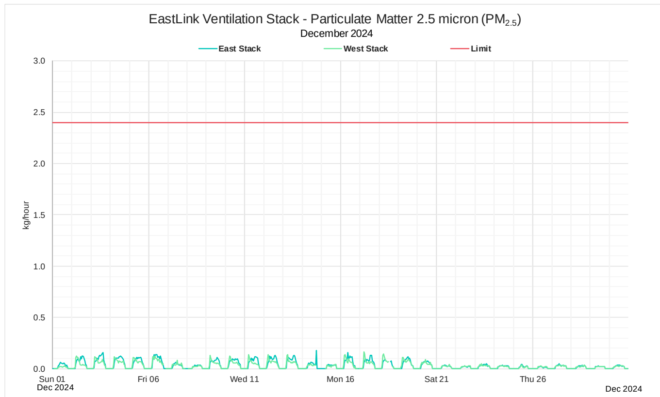
Figure 19: December 2024 Monthly 1-hour mass rate PM_{2.5}
