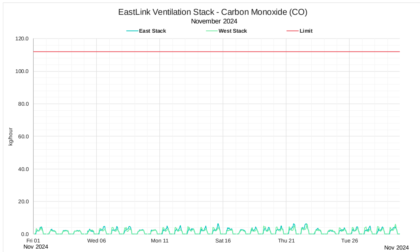
Figure 11: November 2024 Monthly 1-hour mass rate CO
