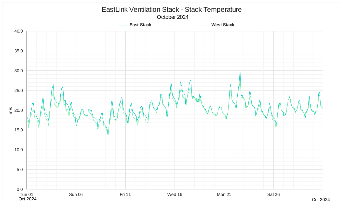
Figure 8: October 2024 Monthly 1-hour average stack temperature
