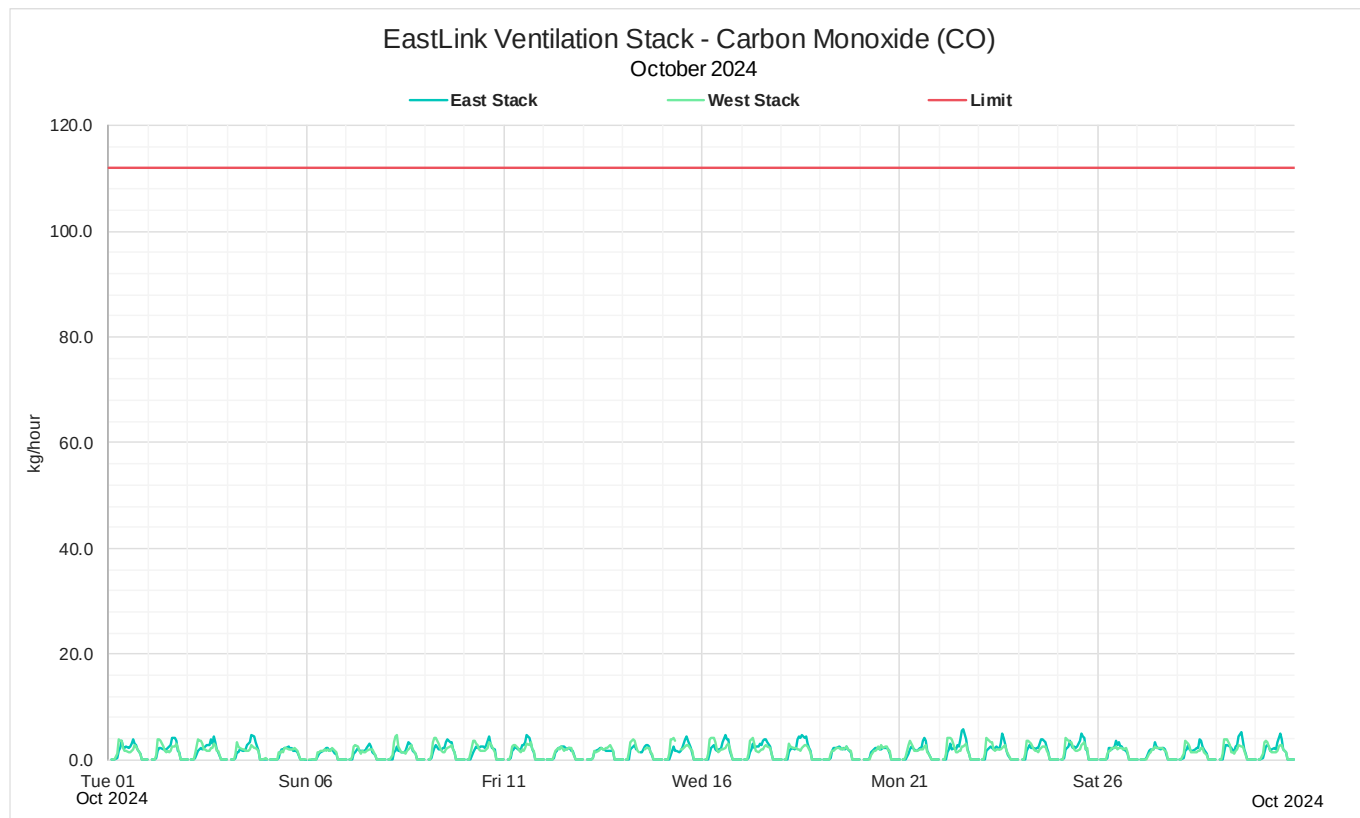
Figure 4: October 2024 Monthly 1-hour mass rate CO
