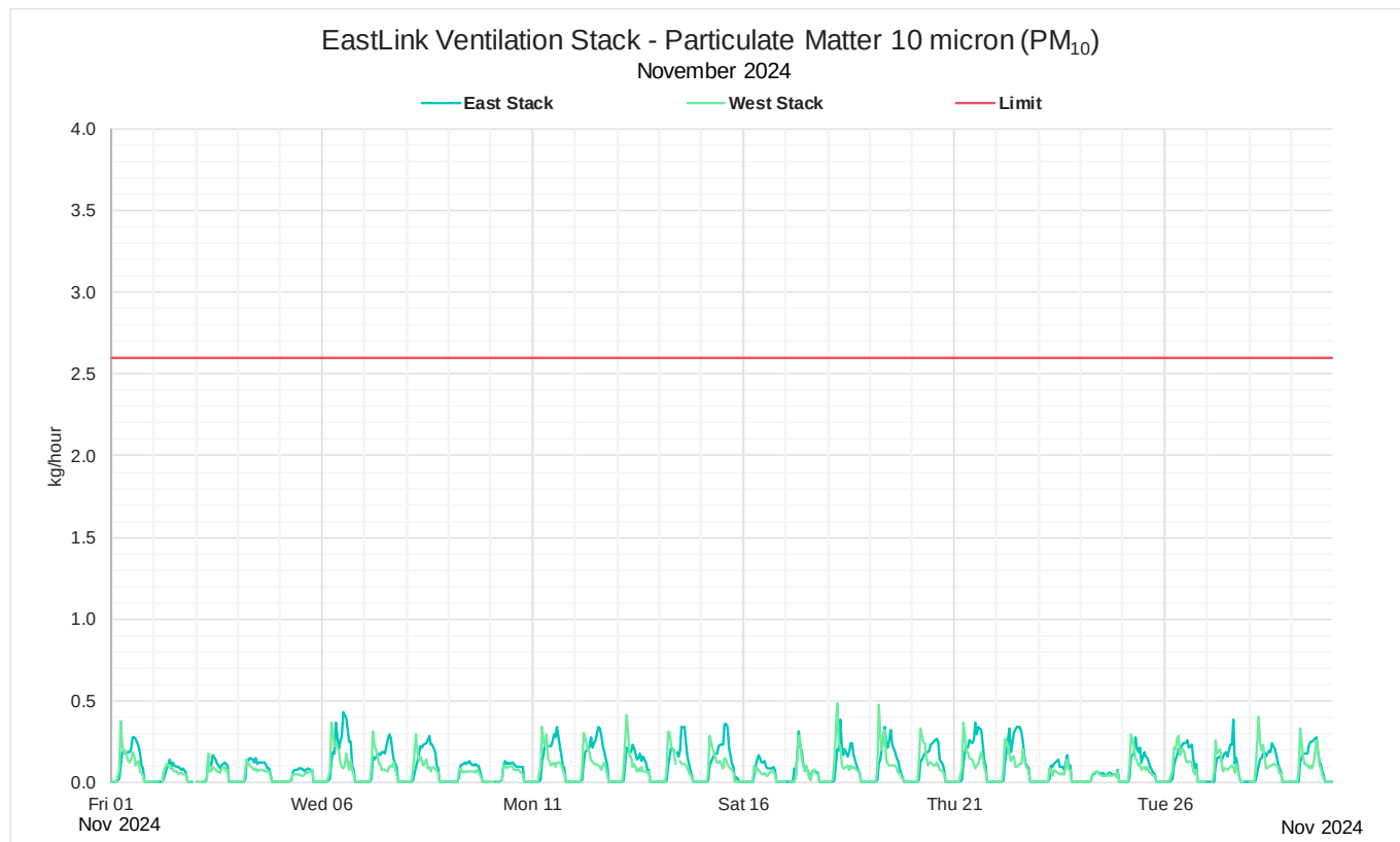
Figure 13: November 2024 Monthly 1-hour mass rate PM_{10}
