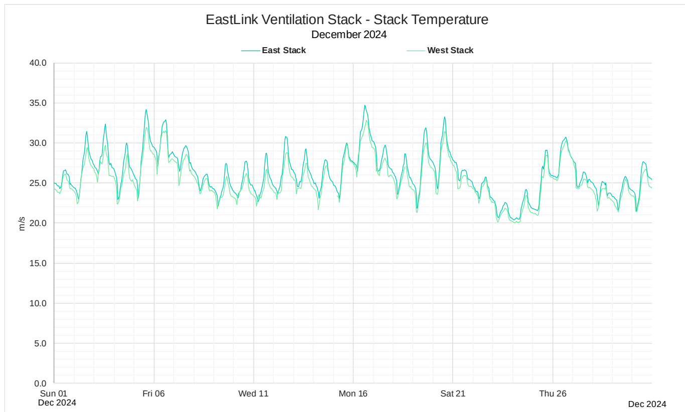
Figure 22: December 2024 Monthly 1-hour average stack temperature
