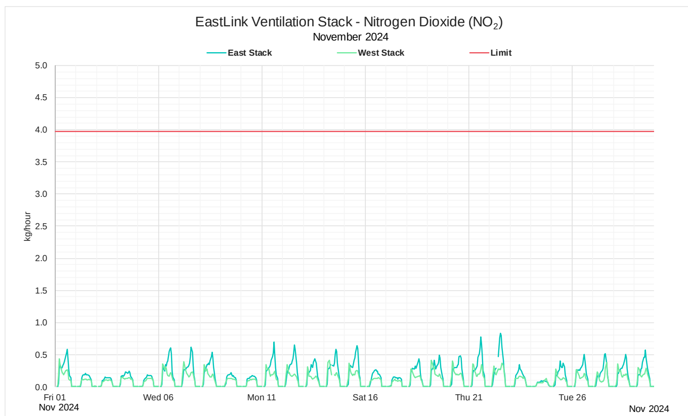
Figure 9: November 2024 Monthly 1-hour mass rate NO 2
